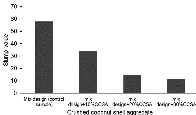
Figure 3. Slump Mean for Concrete Aggregates with CCSA
