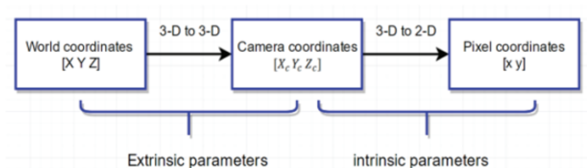
Figure 1. Extrinsic and intrinsic camera parameters (Jackman et al., 2021)
