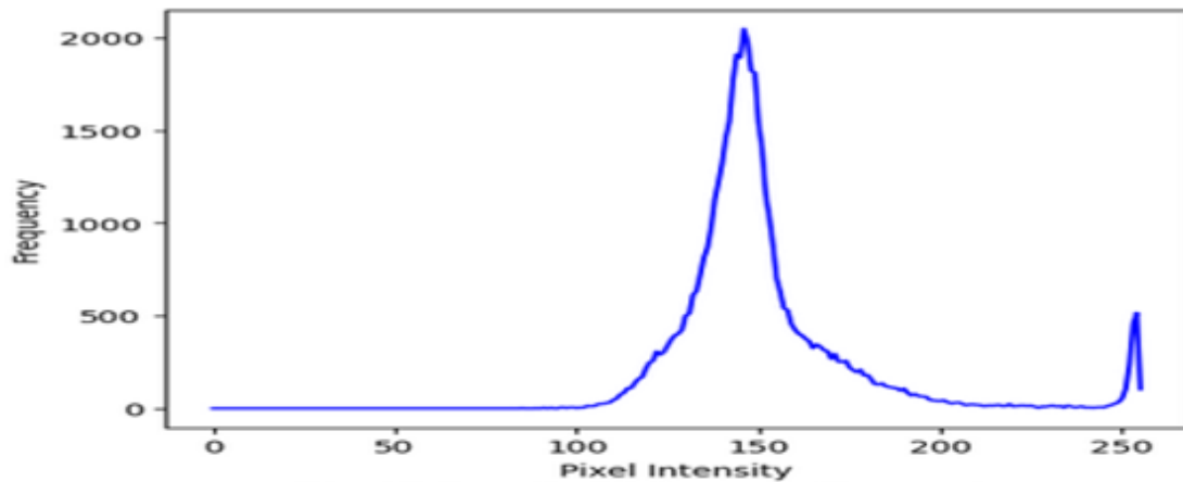
Figure 11. Line graph of pixel intensity for soiled PV panel after 90 days of the experiment
