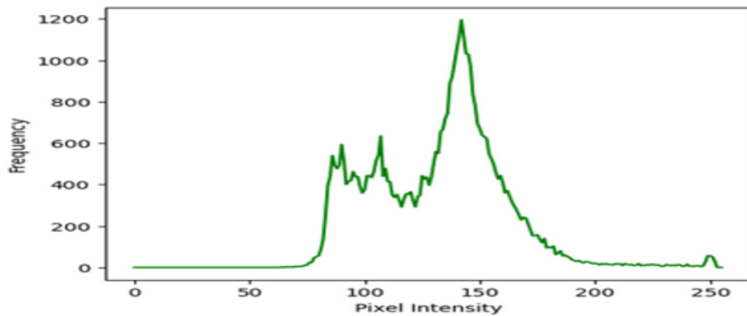
Figure 10. Line graph of pixel intensity for clean PV panel after 30 days of the experiment
