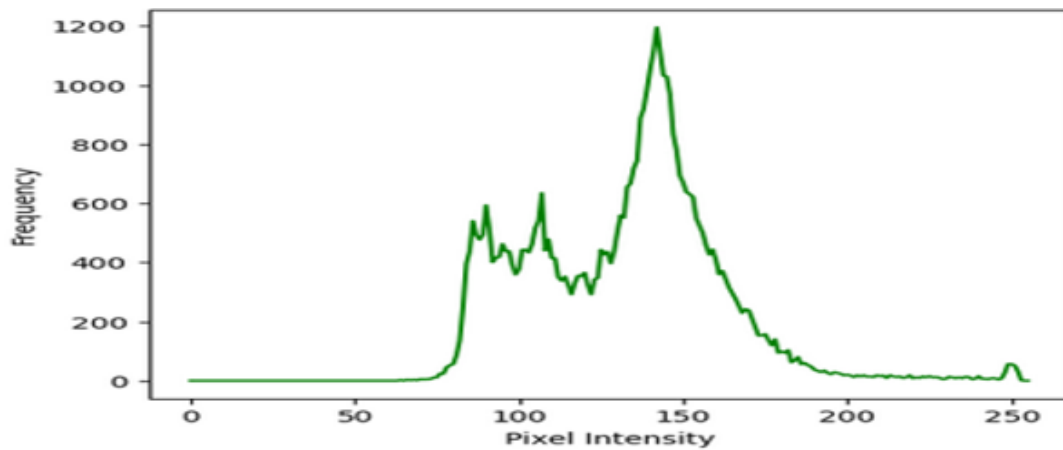
Figure 12. Line graph of pixel intensity for clean PV panel after 90 days of the experiment
