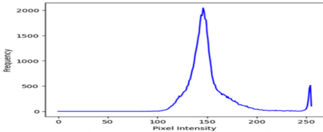
Figure 9. Line graph of pixel intensity for soiled PV panel after 30 days of the experiment
