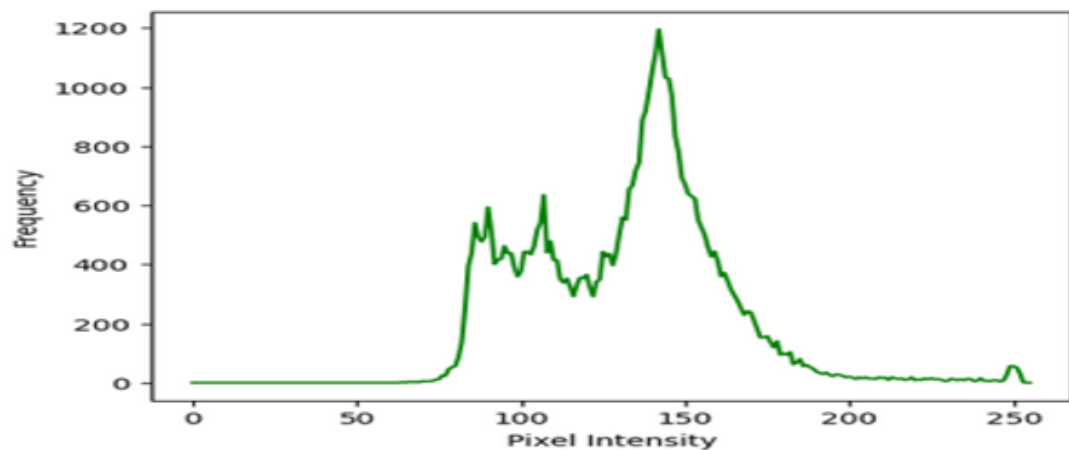
Figure 11. Line graph of pixel intensity for soiled PV panel after 90 days of the experiment
