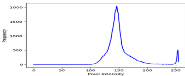
Figure 8. Line graph of pixel intensity for soiled PV panel after 30 days of the experiment Line graphs after 60 Days
