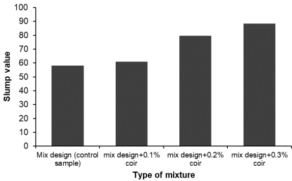
Figure 4. Slump Means for Concrete Aggregates with CCSA
