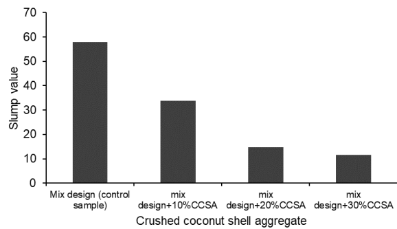
Figure 3. Slump Mean for Concrete Aggregates with CCSA
