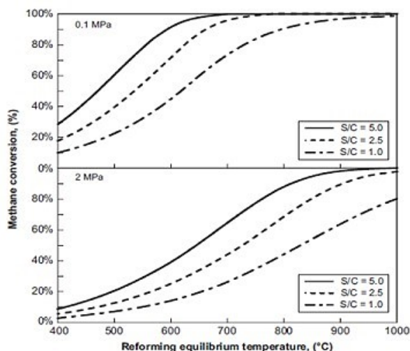
Figure 4. CH 4 Conversion at Different Feed Molar Ratios, Temperature, and Pressure ( Rostrup-Nielsen & Christiansen, 2011 )
