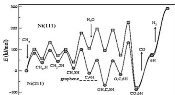
Figure 5. Energy Diagram for Methane Steam Reforming ( Bengard et al., 2002 )
